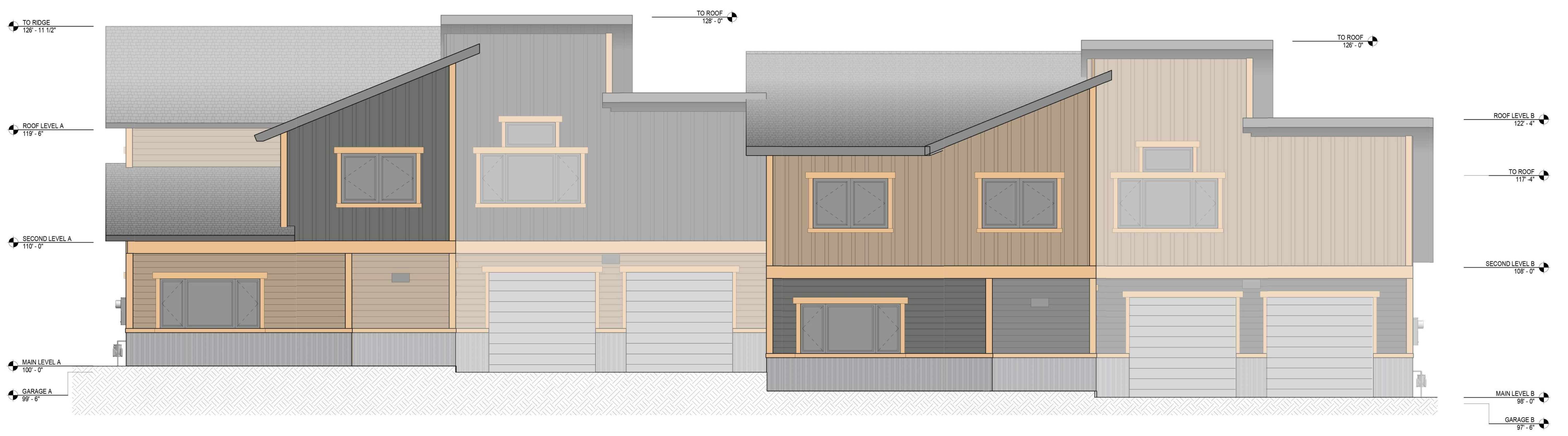
1 SOUTH COLOR OPTION 3 A3.3 1/4" = 1'-0"
