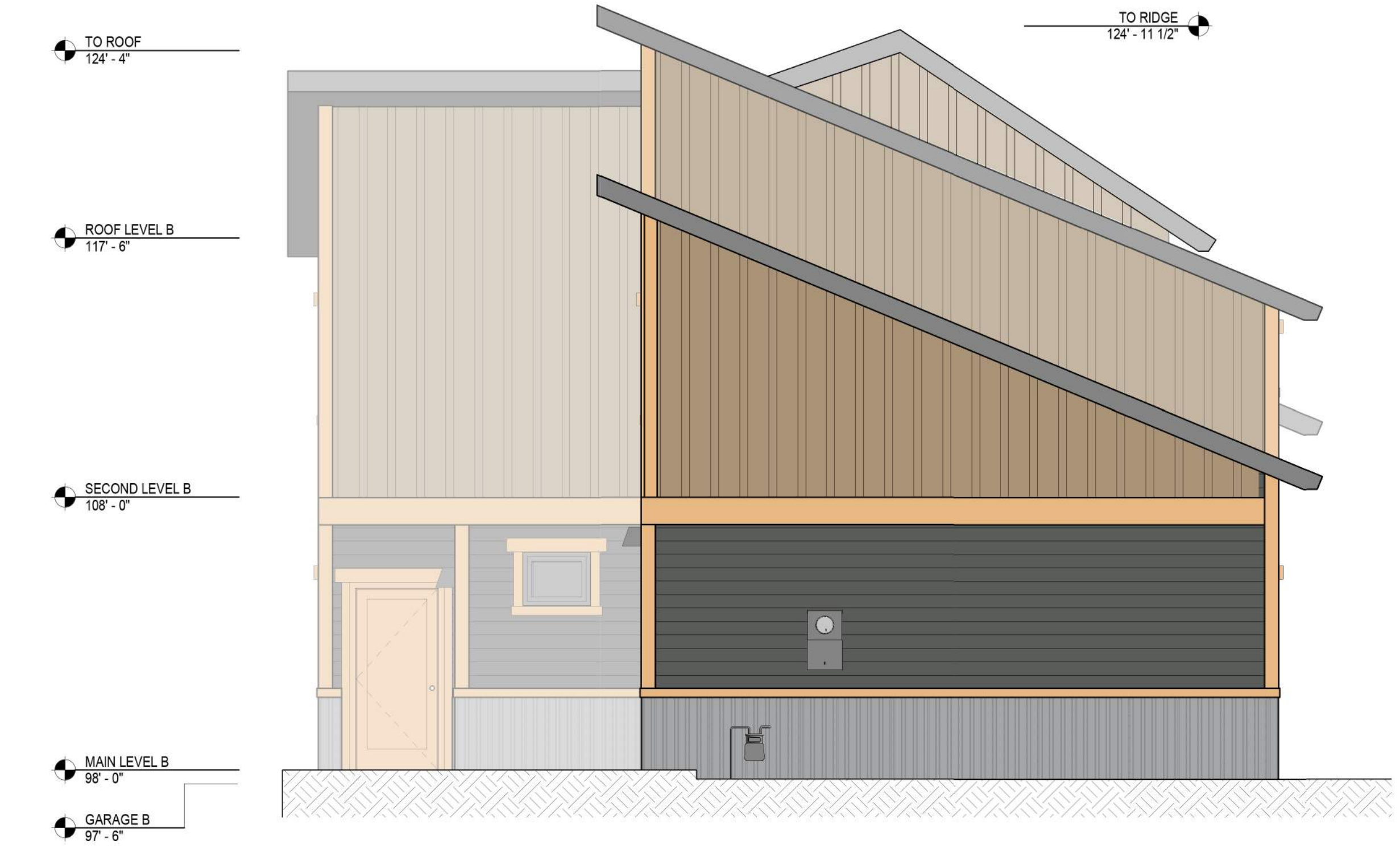
3 EAST COLOR OPTION 3 A3.3 1/4" = 1'-0"
