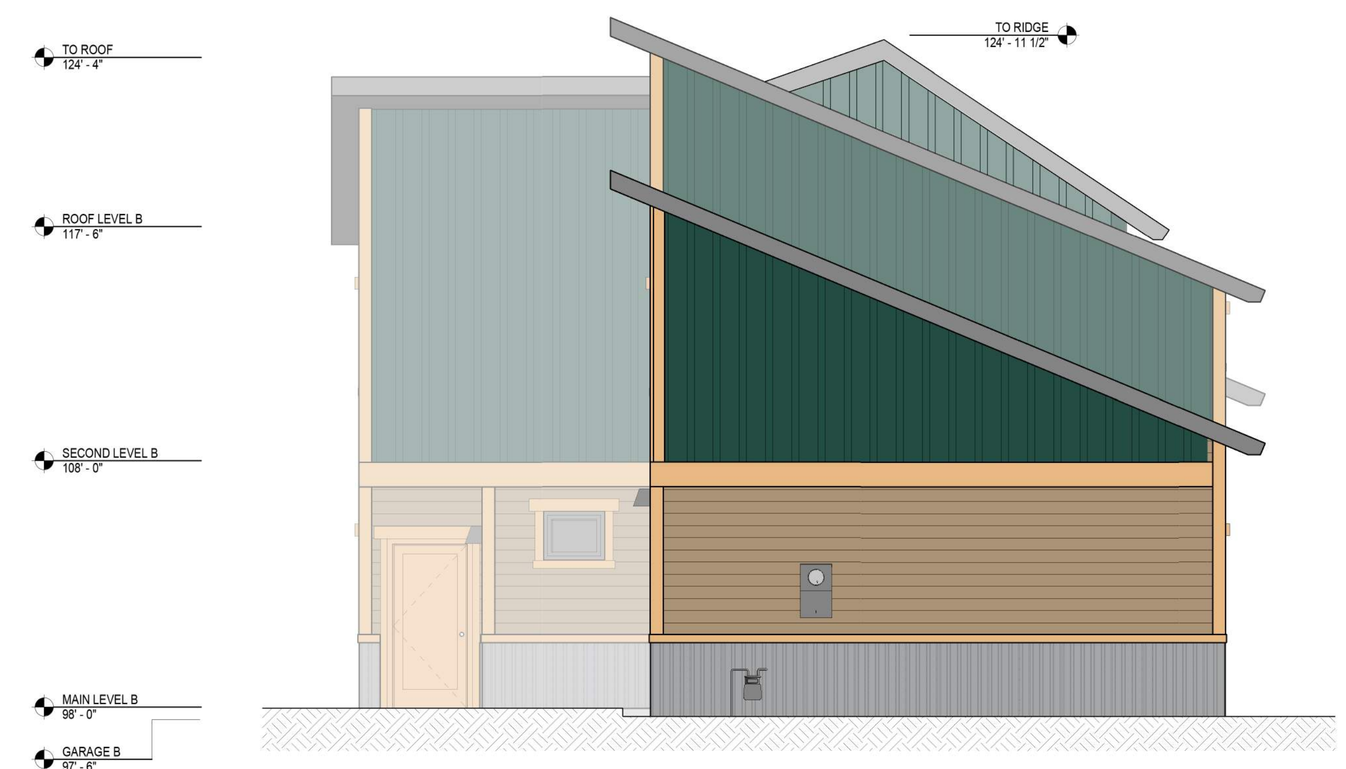
3 EAST COLOR OPTION 2 A3.2 1/4" = 1'-0"
