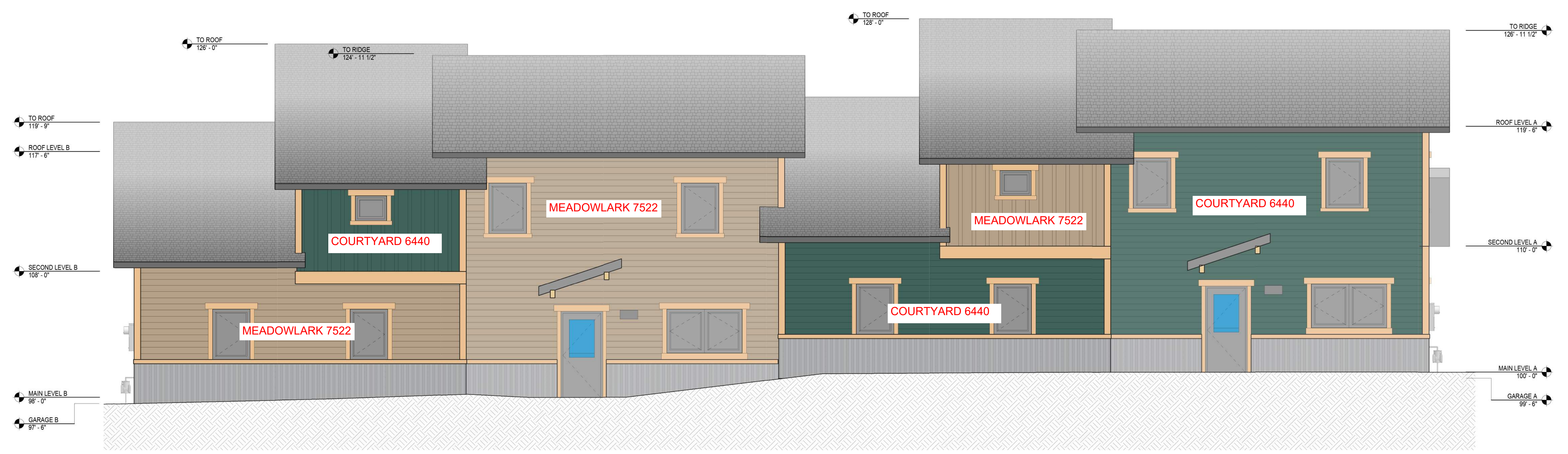
4 NORTH COLOR OPTION 2 A3.2 1/4" = 1'-0"
